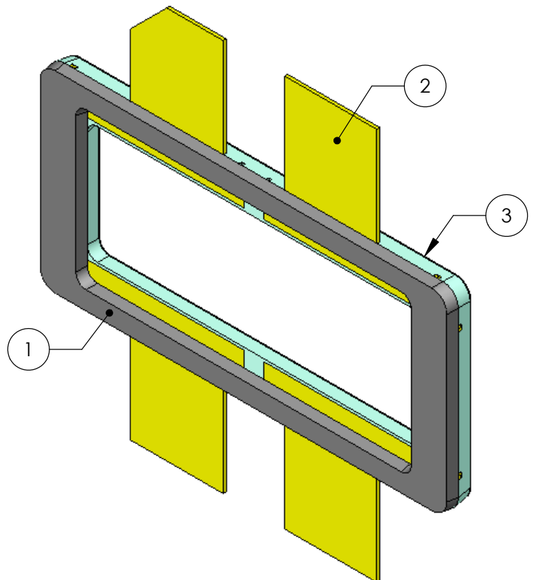
ISOMETRIC VIEW
